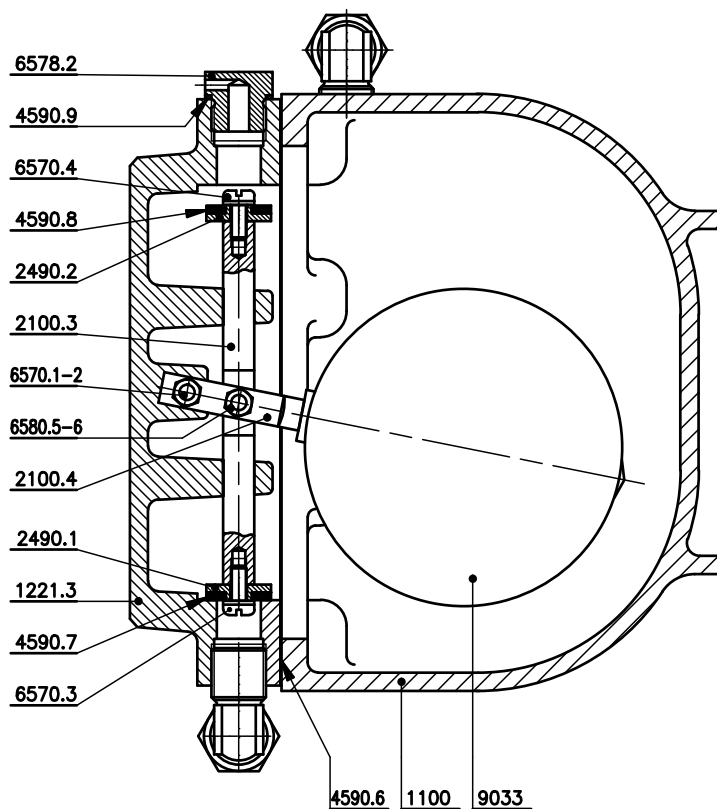
Mechanical purger Purgador mecanico
